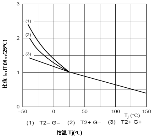
I_{GT}(T_j)/I_{GT}(25°C) - T_j
