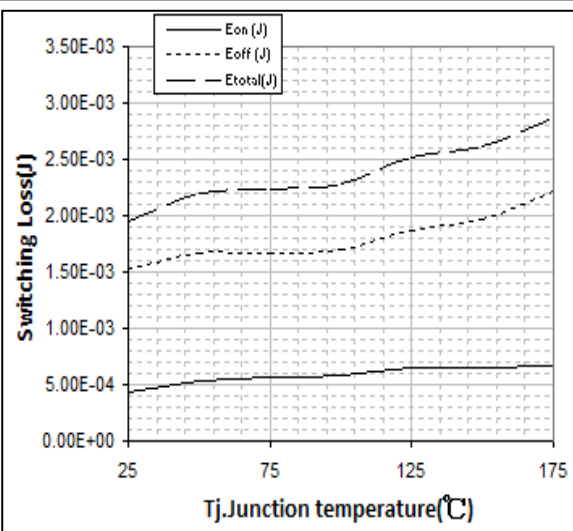
IGBT Switching Loss vs. Tj
