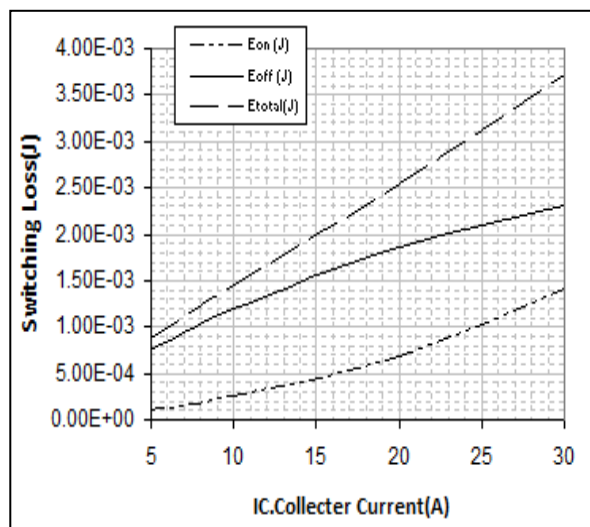
IGBT Switching Loss vs. IC(25°C)
